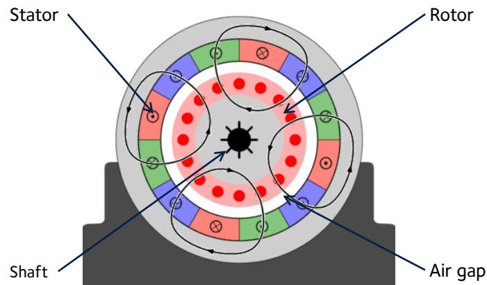
Figure 2: A three-phase induction motor. From [4].
