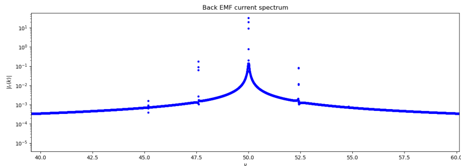
Figure 9: Spectrum of a motor with a defect in one of the rotor loop. \Phi_j = \Phi(1 + 0.1\delta_{j,0})
