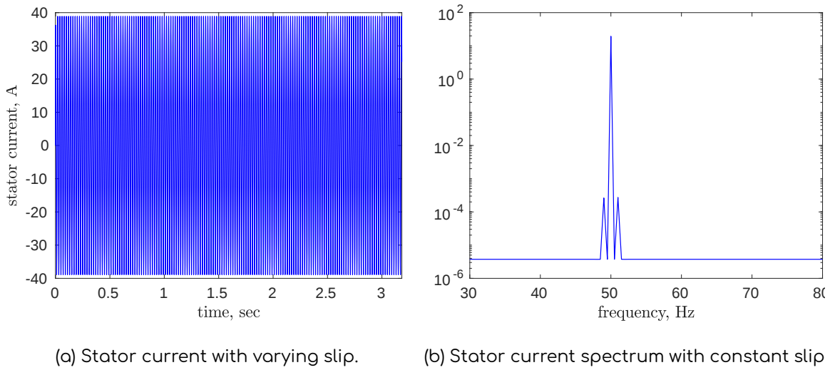
Figure 5: Numerical solution of the variable slip Steinmetz model with parameter values from Table 1.
