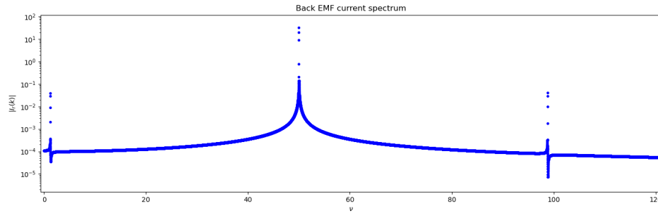
Figure 13: Spectrum of a motor with a time dependant load. \Gamma = 0.2(1 + 0.1 \cos(\theta(t)))
