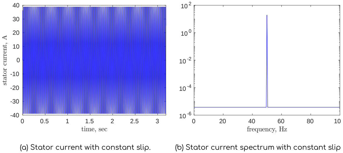
Figure 4: Numerical solution of constant slip Steinmetz model given by (13)–(14) with parameter values from Table 1.
