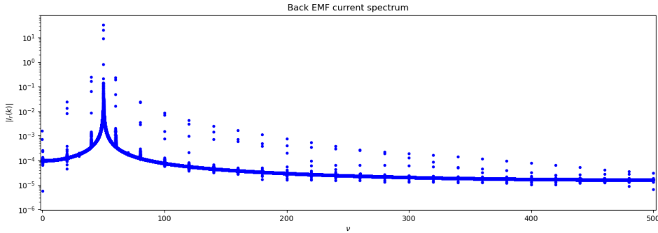
Figure 16: Spectrum of a motor with a time dependant load. \Gamma = 0.2(1 + 0.1SQR(2\pi\nu t)) , \nu = 10Hz , where the SQR function is 1 for the first half of the period and -1 for the second.
