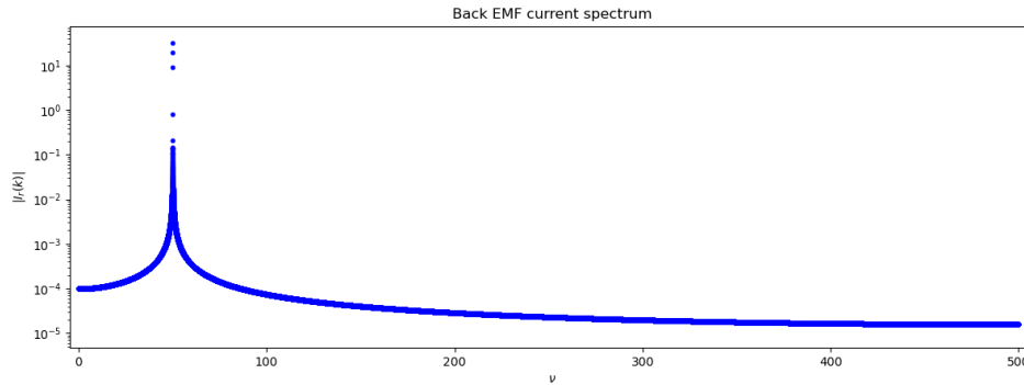
Figure 8: Spectrum of a motor without defect. The spread of the spectrum is due to a non perfect sampling. Slip frequency: 1.22Hz
