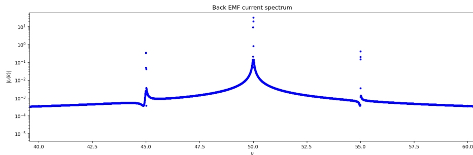
Figure 14: Spectrum of a motor with a time dependant load. \Gamma = 0.2(1 + 0.1 \sin(2\pi\nu t)) , \nu = 5Hz .
